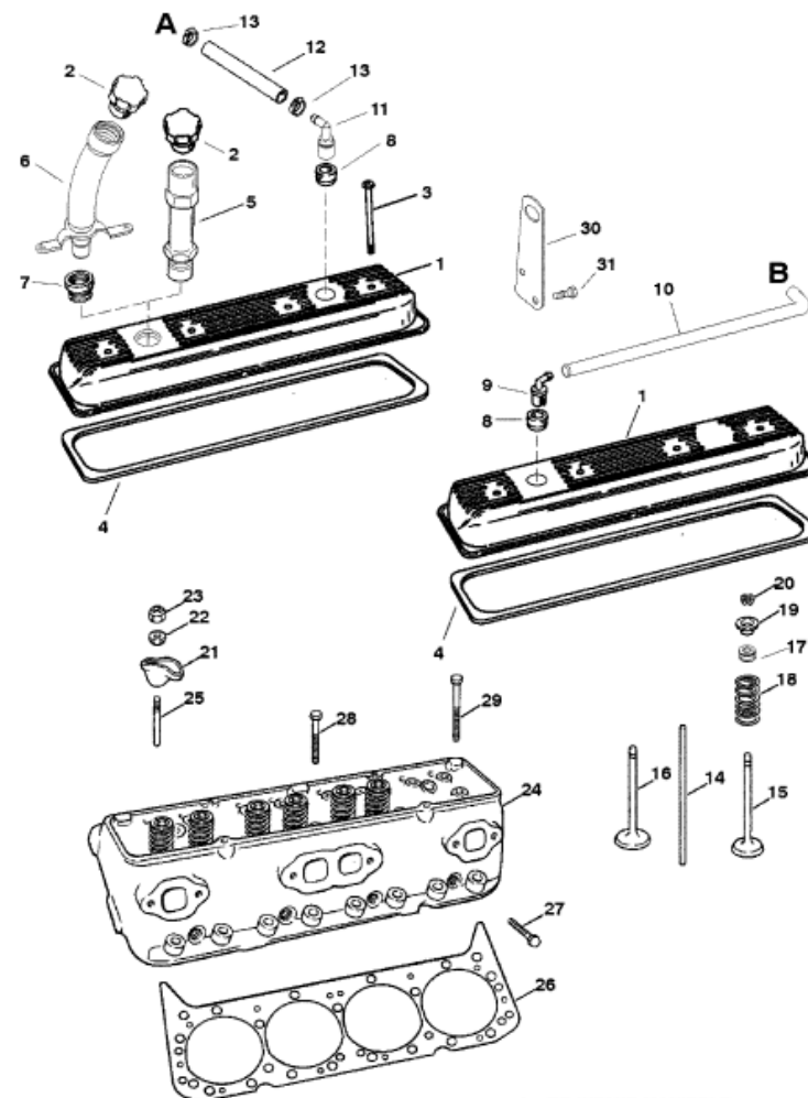
A = TO INTAKE MANIFOLD B = TO FLAME ARRESTOR
